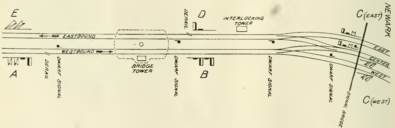
POSITION OF TRACKS, SIGNALS, SWING BRIDGE AND TOWERS ON THE D. L. & W. AT NEWARK, N. J.
